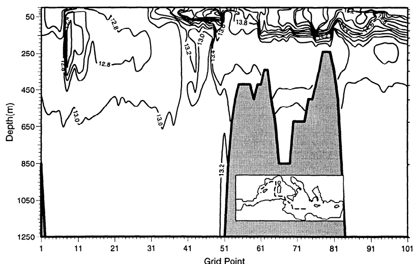
Figure 7. Late wintertime (March) temperature snapshot along a transect (path shown in inset) through the Strait of Sicily, western Mediterranean, and Gulf of Lions for experiment HOL2. The contour interval is 0.2^{\circ}\text{C} .
