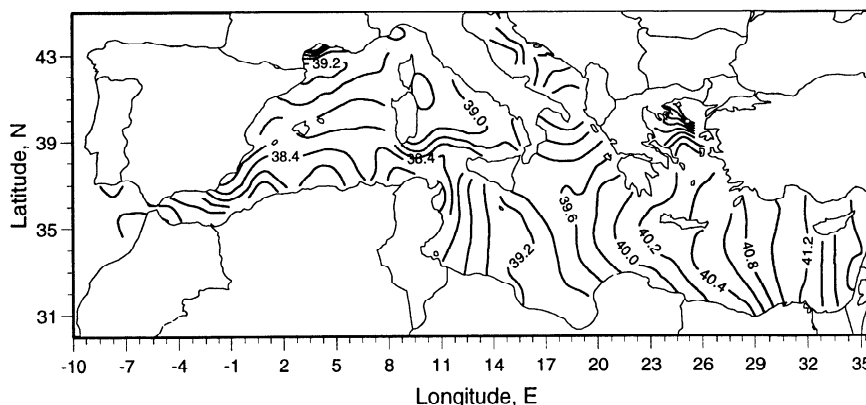
Figure 9. Surface salinity restoring field for the last glacial maximum (LGM) for January for all experiments. The contour interval is 0.2.
