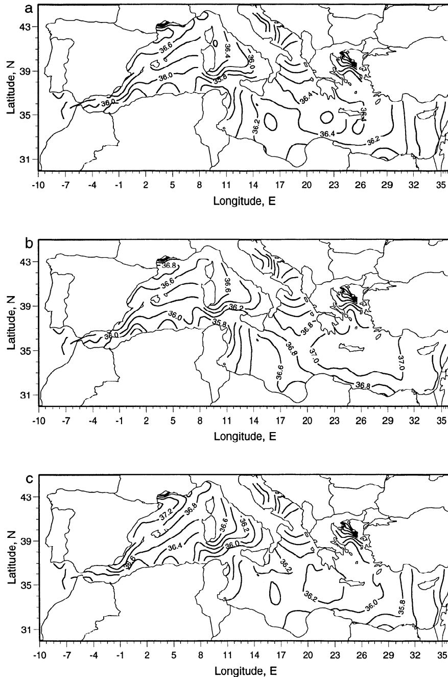
Figure 3. Surface salinity restoring field for the Holocene in January for the reconstructions of (a) HOL1 [Kallel et al., 1987] (b) HOL2 [Rohling and De Rijk, 1998] and (c) HOL3 [Thunell and Williams, 1989]. The contour interval is 0.2.
