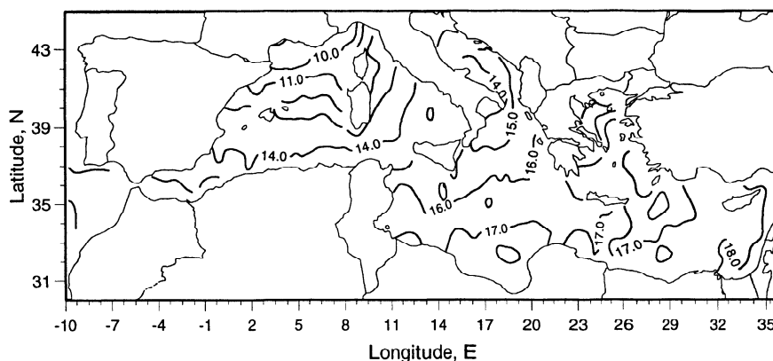
Figure 4. Temperature restoring field for the Holocene for January for HOL4, the reconstruction of Kallel et al. [1997]. The contour interval is 1.0^{\circ}\text{C} .
