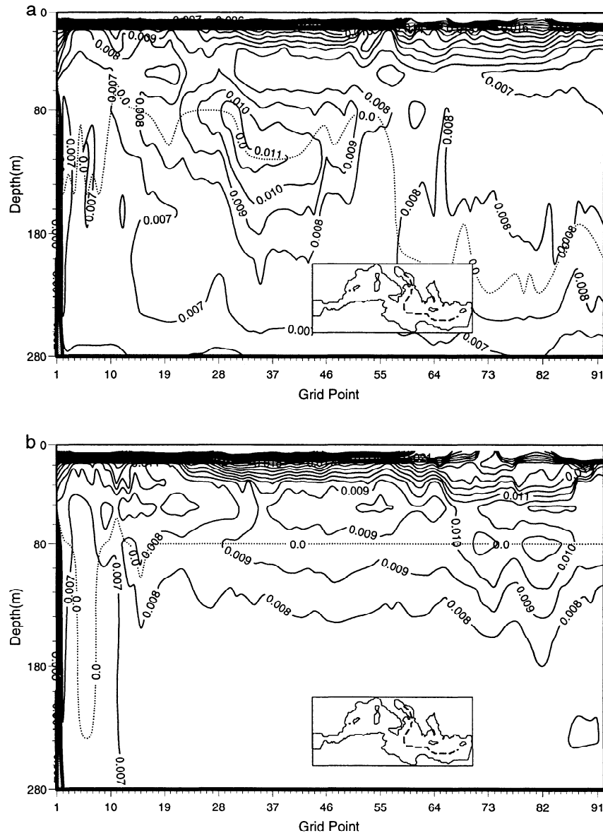
Figure 8. Plot of the Brunt-Vaisala frequency N for an annually averaged transect (path shown in inset) through the eastern Mediterranean and Adriatic showing the depth of the pycnocline for experiments: (a) CONTROL and (b) HOL1. The contour interval is 0.001 \text{ s}^{-1} . The dashed line indicates the approximate position of the model pycnocline (to the nearest model level depth).
