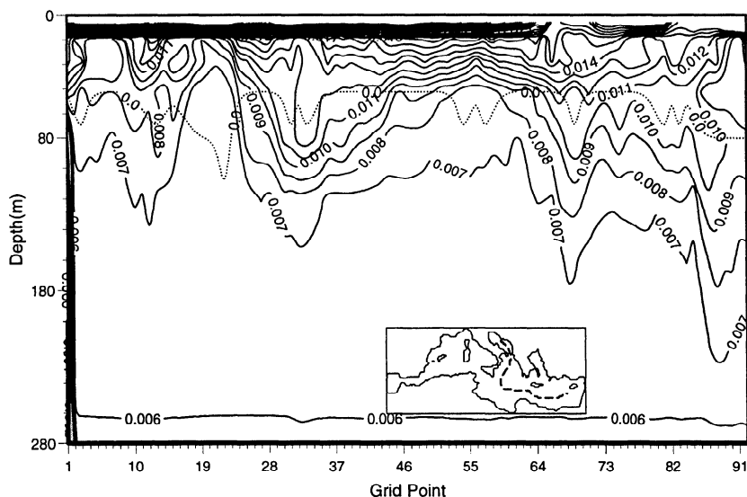
Figure 13. Plot of the Brunt-Vaisala frequency N for an annually averaged transect through the eastern Mediterranean and Adriatic (path shown in the inset) showing the depth of the pycnocline for LGM1 (LGM2 is similar). The contour interval is 0.001 \text{ s}^{-1} . The dashed line indicates the approximate position of the model pycnocline (to the nearest model level depth).
