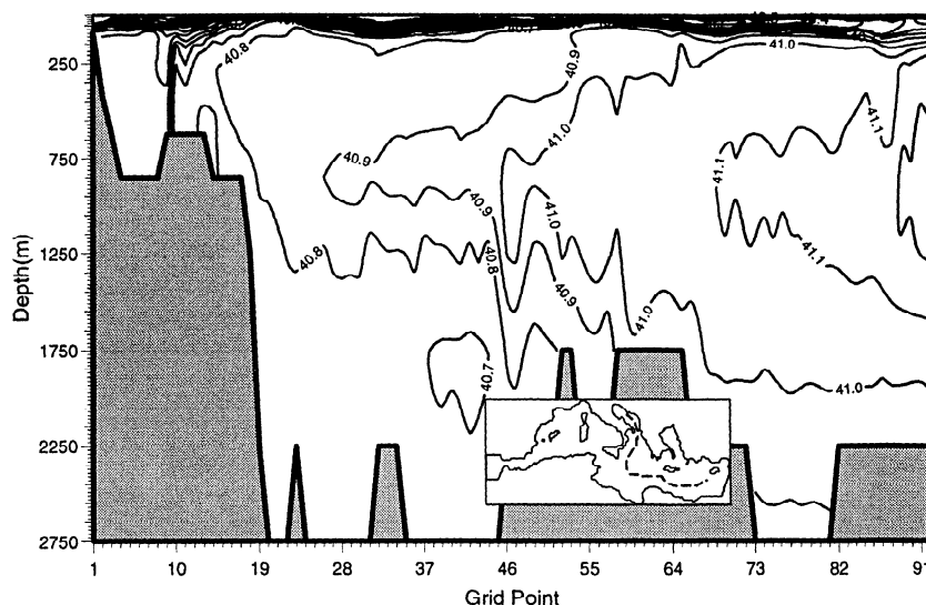
Figure 11. Annually averaged salinity along a transect through the eastern Mediterranean and the Adriatic (path shown in the inset) for LGM1 (LGM2 is similar). The contour interval is 0.1.
