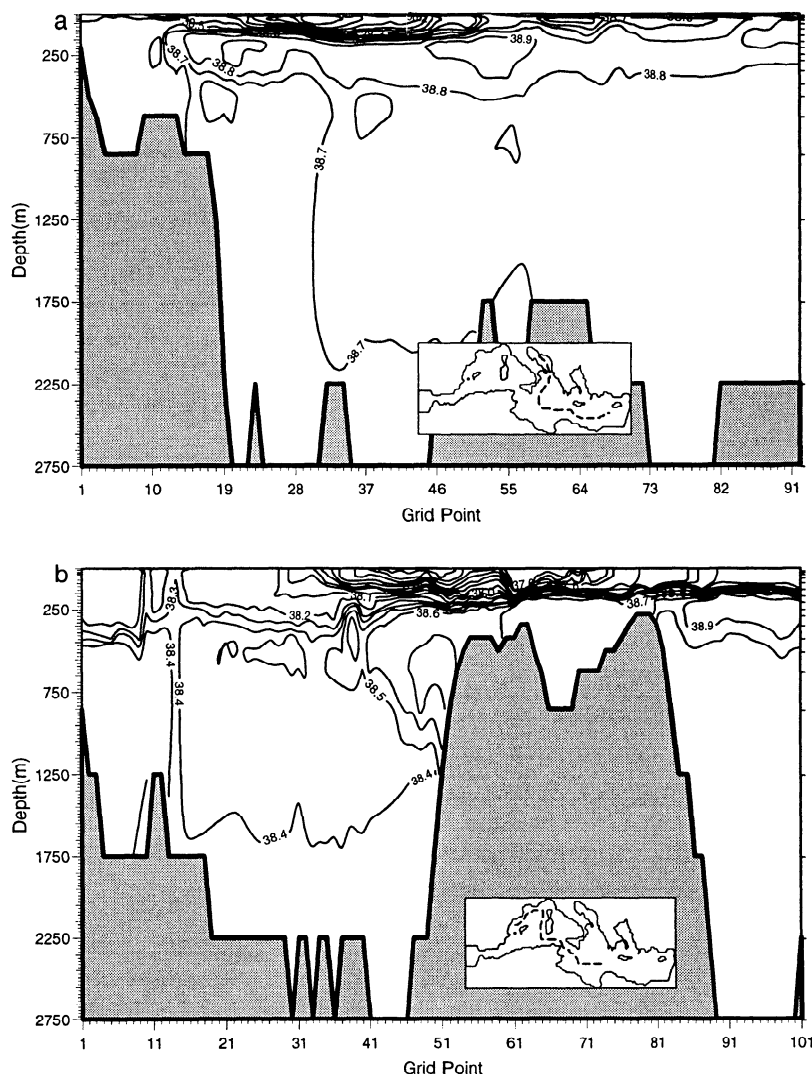
Figure 2. Salinity cross sections for the CONTROL experiment along the paths shown in the inset: (a) annual mean along a transect through the eastern Mediterranean and Adriatic and (b) snapshot along a transect through the Strait of Sicily and the western Mediterranean during late winter (March). The contour interval is 0.1 in both.
