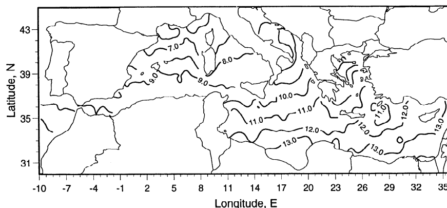
Figure 10. Surface temperature restoring field for LGM2 for January. The contour interval is 1.0°C.
