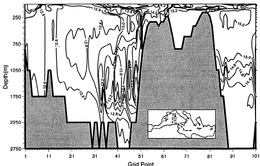
Figure 12. Late wintertime (March) temperature along a transect through the Tyrrhenian and the Gulf of Lions (path shown in the inset) for LGM1. The eastern basin is to the right. The contour interval is 0.2°C.
