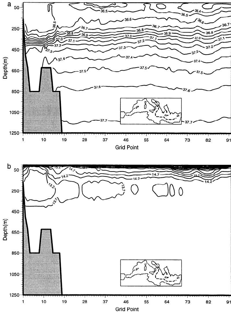
Figure 5. Annually averaged (a) salinity and (b) temperature along a transect (path shown in inset) through the eastern Mediterranean and Adriatic for experiment HOL1 [Kallel et al. , 1997]. The contour interval is 0.1 in Figure 5a and 0.5°C in Figure 5b.
