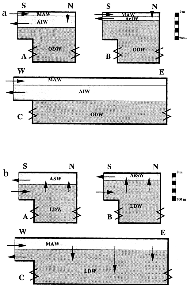
Figure 14. Schematic summarizing the results of our model experiments for the (a) Holocene and (b) LGM, with the locations of the sections shown in Figure 1. The abbreviations for the water masses are AIW, Adriatic Intermediate Water; ODW, Old Deep Water; AeIW, Aegean Intermediate Water; ASW, Adriatic Surface Water; AeSW, Aegean Surface Water; MAW, Modified Atlantic Water; and LDW, Levantine Deep Water.
