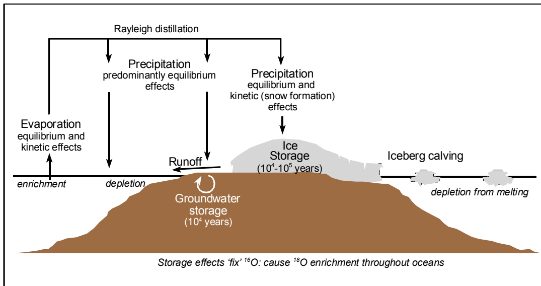
Figure 1. Schematic presentation of the hydrological cycle influences on oxygen isotope ratios. Effects on seawater are described in italics (after Rohling and Cooke, 1999). The “fix” comment refers to the storage of preferentially ^{16}\text{O} enriched precipitation in ice sheets and groundwater, which constitutes a preferential removal of ^{16}\text{O} from the oceans and thus a relative ^{18}\text{O} enrichment in the oceans.
