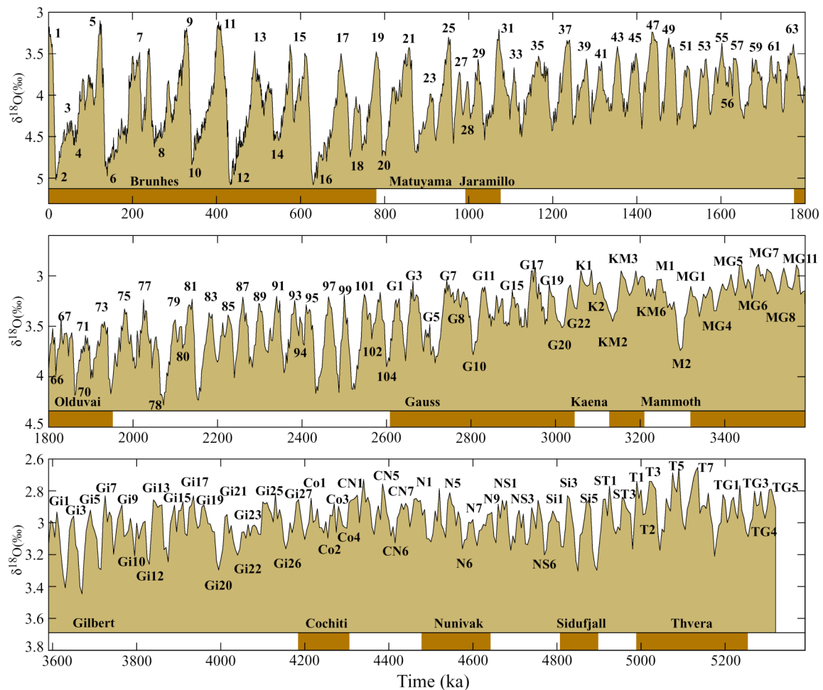
Figure 4. A stacked record of stable oxygen isotope variations for the last 5.3 million years, constructed from 57 globally distributed deep-sea (benthic foraminiferal) records. Numbers indicate glacial (down = heavy \delta^{18}\text{O} values) and interglacial (up = light \delta^{18}\text{O} values) intervals. The dark/light bar at the bottom of each panel indicates (named) intervals of normal (dark) and reversed (light) geomagnetic polarity. Time is indicated in units of one thousand years (ka). After Lisiecki and Raymo (2005).
