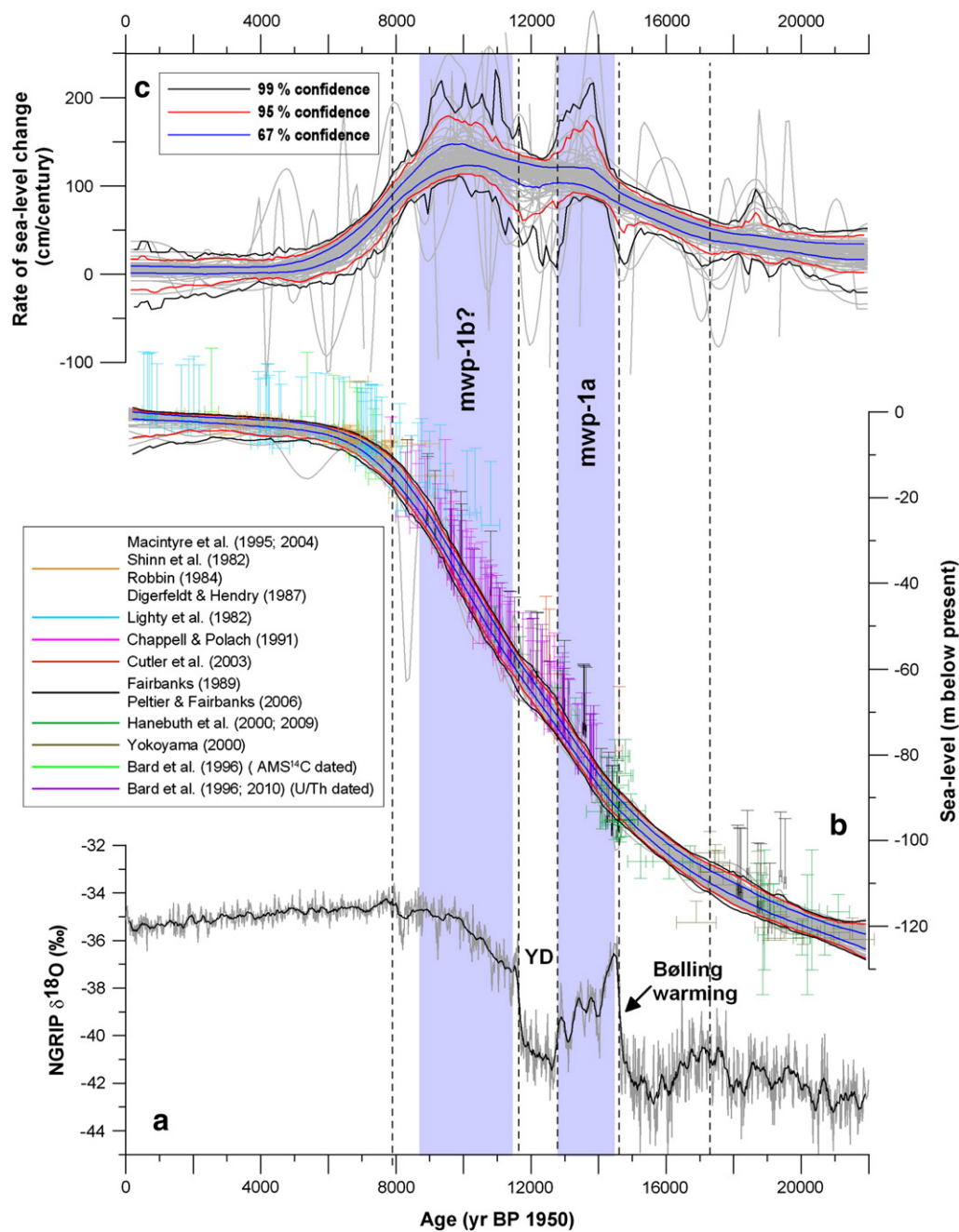
Fig. 4. Same as in Fig. 3, except a 15 m depth uncertainty for the corals was used.
