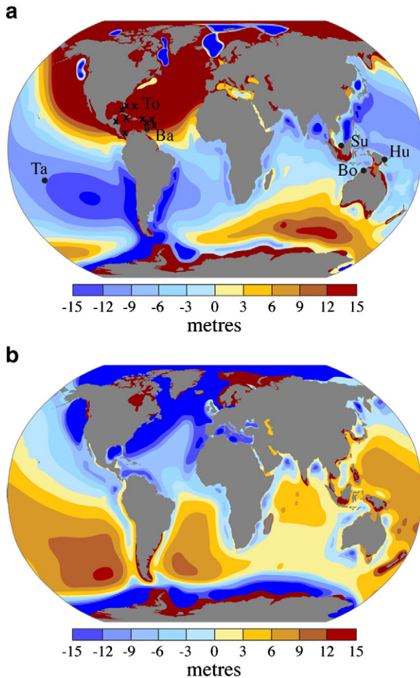
Fig. 1. The predicted total relative sea level (RSL) change minus the model eustatic component for a time window extending from 21 ka BP (a) and 6 ka BP (b) to the present-day. These predictions (departures from the eustatic change) are reproduced from Milne and Mitrovica (2008), who used the Basset et al. (2005) ice model and associated Earth model in their study. The ice and Earth model produced an optimal fit to a number of far-field records. The zero contours show where RSL is equal to the modelled eustatic value. The red and blue colours indicate where sea-level is greater or less than the eustatic value. Ta = Tahiti, Ba = Barbados, Bo = Bonaparte Gulf, Su = Sunda Shelf and Hu = Huon Peninsula. Crosses show the location of datasets used in the Toscano and Macintyre (2003) compilation.
