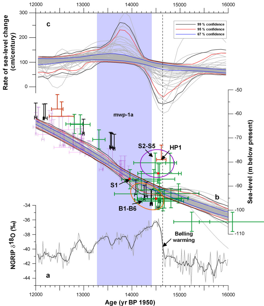
Fig. 7. Same as Fig. 3, but for the time period 12 to 16 ka BP. The datasets discussed in the main text are highlighted by thicker symbols. Red asterisks denote the mean ages of in situ mangrove root samples from the Sunda Shelf. Numbered samples are those that lie outside the 99% confidence limits and are discussed in the main text.
