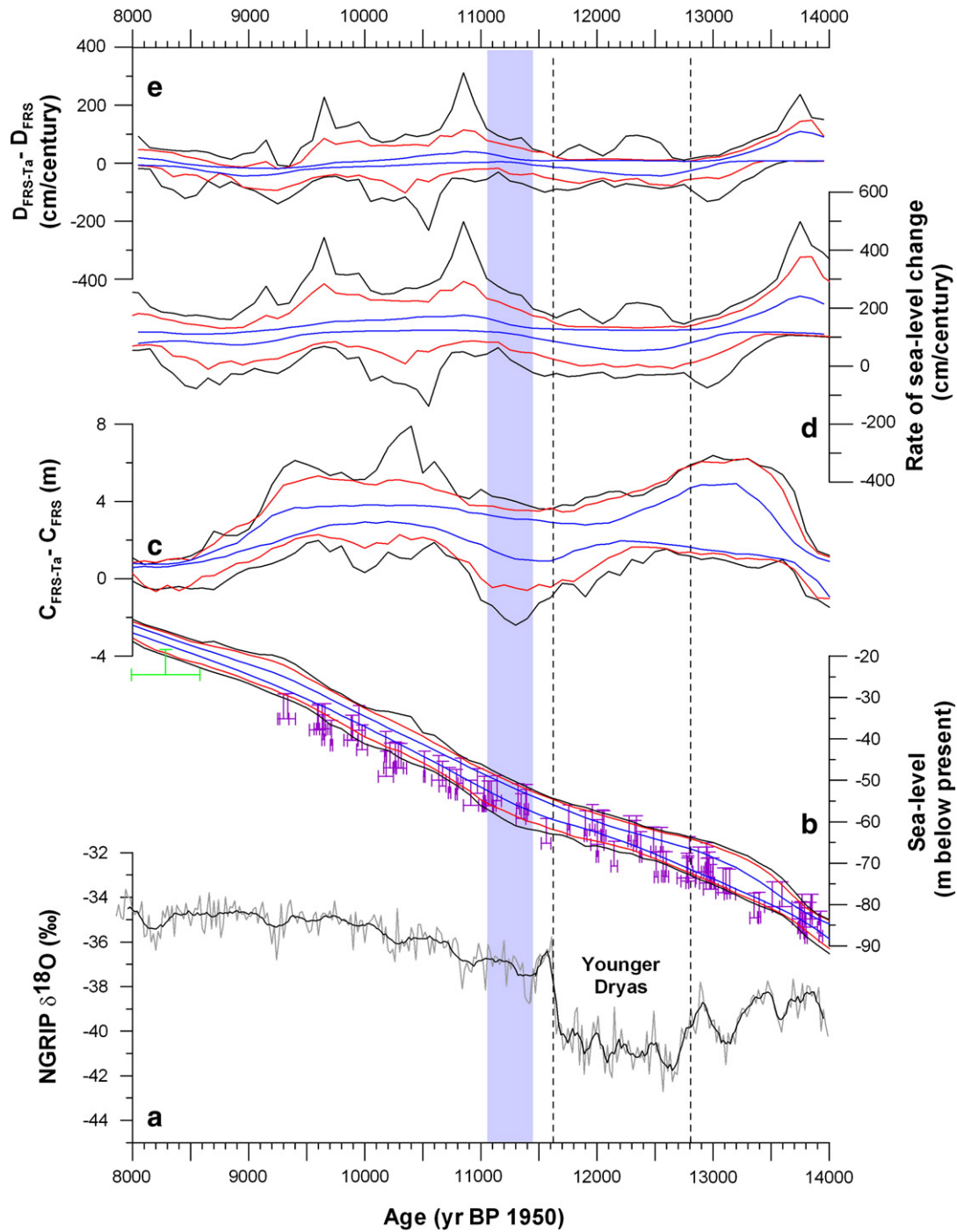
Fig. 6. Same as Fig. 5D, but for 8 to 14 ka BP.
