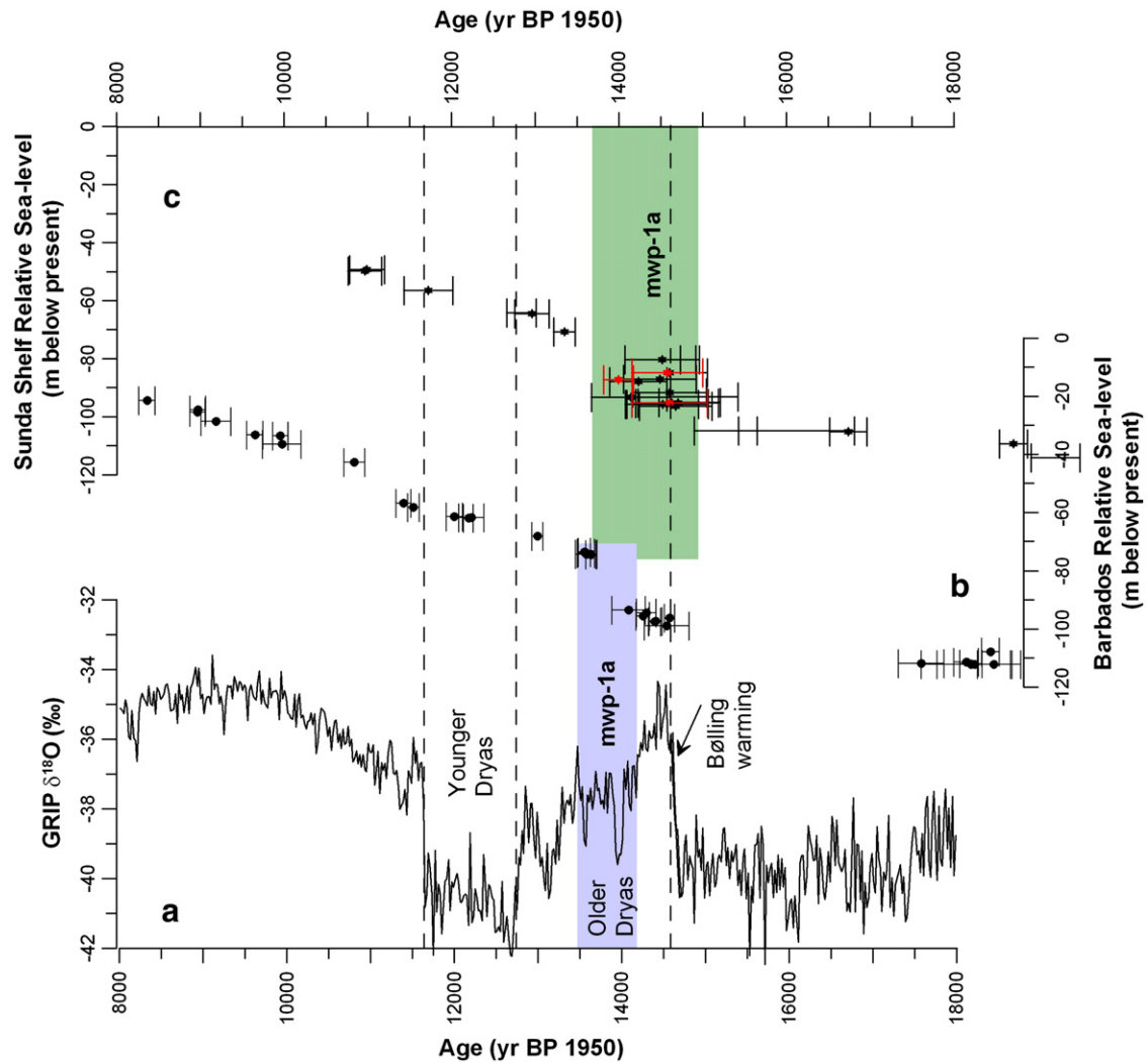
Fig. 2. a. The GRIP ice core \delta^{18}\text{O} record on the GICC05 timescale on the basis of layer-counting (Andersen et al., 2006; Svensson et al., 2006; Rasmussen et al., 2006, 2008). b. The U/Th-dated Acropora palmata corals from Barbados in black, which are corrected for a constant tectonic uplift of 0.34 \text{ m kyr}^{-1} (Fairbanks et al., 2005; Peltier and Fairbanks, 2006). c. The ^{14}\text{C} dated Sunda Shelf sea level record (re-calibrated from Hanebuth et al., 2000). Symbols indicate the mean ages and those that are plotted with only their 2\sigma error bars represent ages with calibrated multiple 1\sigma probabilities. Datings on in situ roots and root fibres from the Sunda Shelf are shown in red, with their 2\sigma error bars. The green and blue bars represent the inferred timings of mwp-1a from the Sunda Shelf and Barbados sea-level records, respectively.
