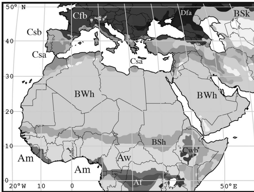
Figure 1. Summary map of the main climate zones in the study region using the Köppen-Geiger climate classification. A = equatorial; B = arid; C = warm temperate; D = snow; s = summer dry; f = fully humid; S = steppe; W = desert; w = winter dry; m = monsoonal; a = hot summer; b = warm summer; k = cold arid; h = hot arid. Modified after Kottek et al. (2006). A color version of this figure is available in the online edition of Current Anthropology .
