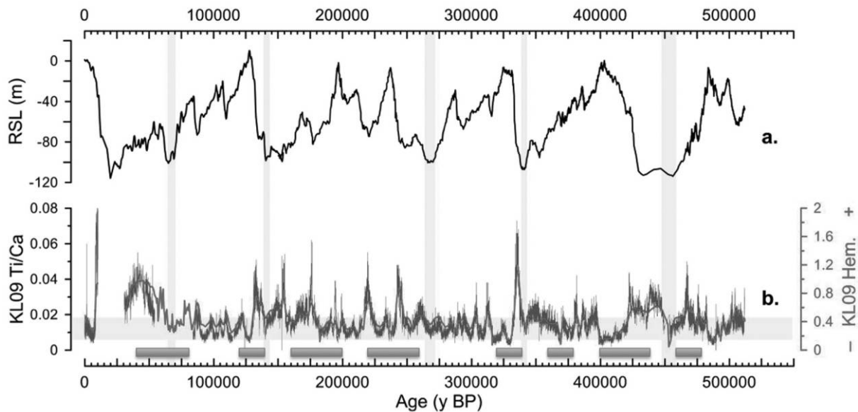
Figure 8. Direct comparison between (a) the latest version of the Red Sea sea-level reconstruction, with the pre-150 ka interval on the chronology of Rohling et al. (2009b, 2010) and the post-150 ka interval on the new chronology of Grant et al. (2012), and (b) central Red Sea dust proxy data, including the Ti/Ca ratio from core-scanning XRF analysis (gray) and hematite concentration data from environmental magnetic analyses (smooth line; see also Roberts et al. 2011; Rohling et al. 2008a). Data originate from a single sampling of the same sedimentary sequence, which ensures unambiguous phase relationships between the various records. Light gray bars are explained in the text. Horizontal bars at bottom indicate intervals of particularly pronounced millennial-scale climate variability, after the analysis of Siddall et al. (2010; see also fig. 7). A color version of this figure is available in the online edition of Current Anthropology .
