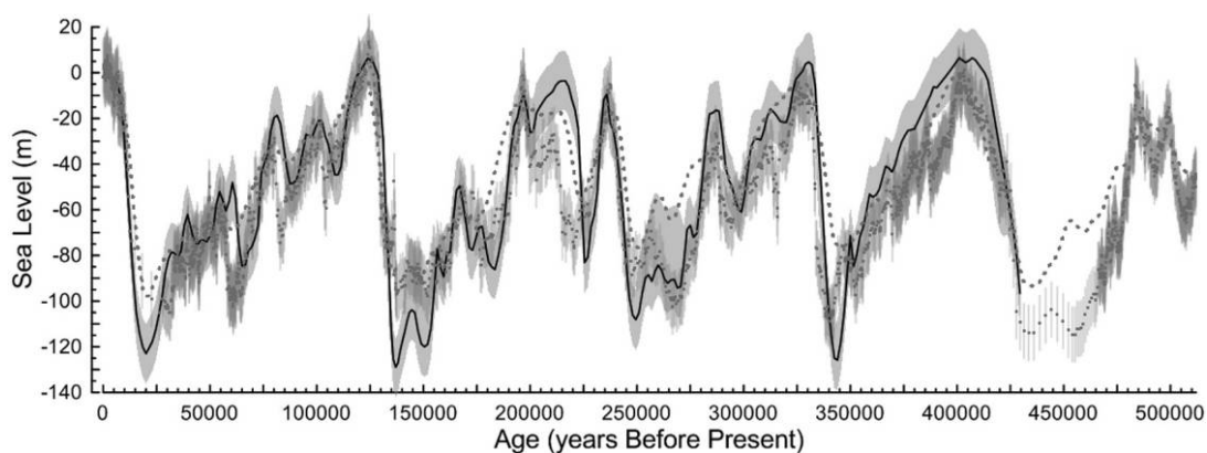
Figure 4. Comparison between three approaches for reconstructing continuous records of sea-level variations. Black is Waelbroeck et al. (2002), based on coral-calibrated deep-sea stable oxygen isotope data, with uncertainties in gray. The dashed line is the reconstruction of De Boer et al. (2010, 2011) from a model-based deconvolution of deep-sea stable oxygen isotope records into a temperature and a sea-level component following the method of Bintanja, van de Wal, and Oerlemans (2005). Dots with ( 2\sigma ) uncertainty bars represent the Red Sea reconstruction on a U-Th-adjusted chronology (Rohling et al. 2009 b , 2010). Modified after Rohling et al. (2012). A color version of this figure is available in the online edition of Current Anthropology .
