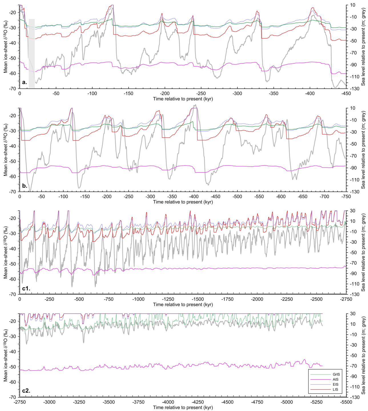
Supplementary Figure S5. Weighted mean ice-sheet \delta^{18}\text{O} for the various ice sheets ( \overline{\delta_{ice}} ). For sea level based on: a. the Red Sea record (8,9,10,11); b. sea-level stack (12); c1 and c2. the benthic \delta_c stack (13) (main case regression, Suppl. Fig. 3). Panel c is divided into younger ( c1 ) and older ( c2 ) halves, for clarity.
