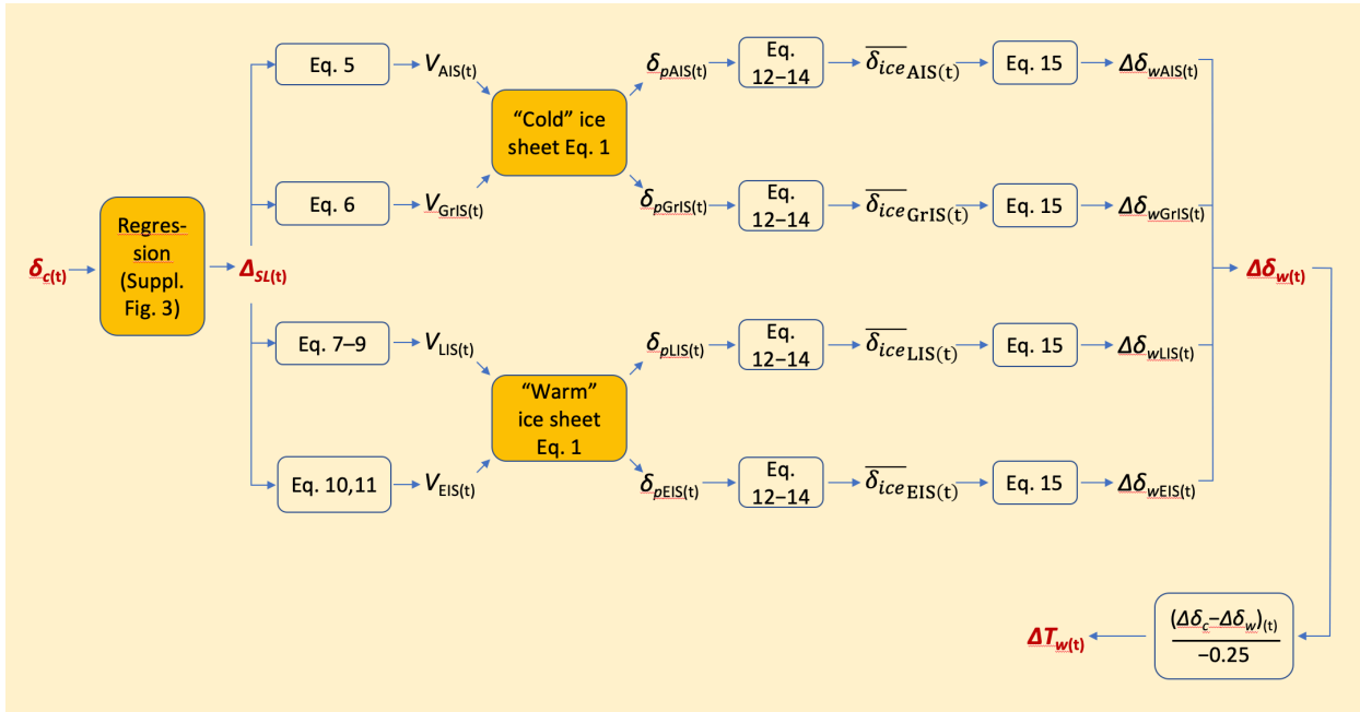
Supplementary Figure S2. Diagram of the workflow used in our applied assessments. Equation numbers refer to the Methods section. Subscript (t) is given to indicate parameter development through time. Red highlights indicate the main parameters of interest between which we investigate mutually consistent relationships. It is evident from the left-to-right progression that there are no circularities in the method. Darker yellow boxes indicate stages where the main assumptions are made. One assumption concerns the regression-based approach to derive \Delta_{SL} from \delta_c (Suppl. Fig. S3). Sensitivity tests with different regressions indicate that the \Delta_{SL} solution is robust within a total uncertainty range of about 10 m (i.e., if a mean were chosen from the three solutions, then uncertainties would span up to \pm 5 m at 99% confidence). This robustness is emphasized by the multi-parameter validations undertaken here. Another assumption concerns the shape of the \delta_p relationships with ice volume. Sensitivity tests with alternative contrasting (linear) relationships indicate that our main conclusions are affected little by the relationship shape (Fig. 1).
