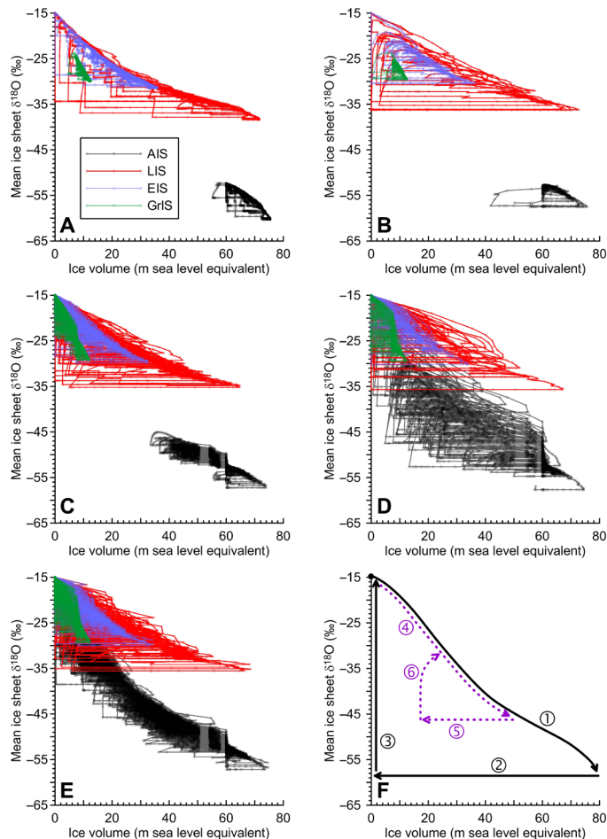
Fig. 5. Diagrams of \delta_{ice} relative to ice sheet volume for individual ice sheets for the five main model runs investigated in this study. (A) Sea level record based on the Red Sea method (8–11), (B) sea level stack (12), (C) benthic \delta_c stack-based sea level record (main regression in fig. S3) (13), (D) sea level record from the Mediterranean Sea method (46), and (E) youngest 40 Ma of the benthic \delta_c megaspline-based record (main regression in fig. S3) (14). The less complete V_{ice}\delta_{ice} representations are for shorter records that do not cover the full bipolar ice sheet response range; the more detailed (D) and (E) are more representative. The greater noise in (D) results from lower precision of the Pliocene Mediterranean \Delta_{SL} record. (F) Schematic illustration of the nature of the relationships in (A) to (E). In (F), 1 represents the trajectory associated with gradual ice-volume buildup, determined by continuous instantaneous ice volume–based adjustment of \delta_p , and lagged adjustment of \delta_{ice} according to the residence-time calculation discussed in Methods (Eqs. 12 to 14). 2 represents rapid ice loss during deglaciation that occurs at the \delta_{ice} value attained just before deglaciation onset; and 3 represents adjustment at the end of deglaciation, when new ice starts to build up at the starting \delta_p value. 4 is the trajectory associated with gradual partial deglaciation (as 1), 5 is rapid partial deglaciation (as 2), and 6 represents more gradual \delta_{ice} adjustment to conditions commensurate with the remaining ice volume after partial deglaciation.
