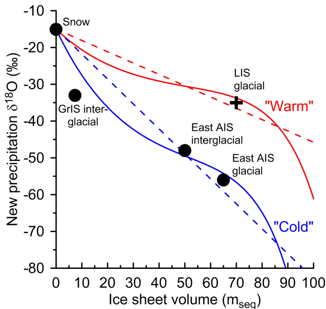
Supplementary Figure S1. Shape of the \delta_p versus ice-sheet volume relationships used in our analytical and applied assessments. Blue indicates lines used for AIS and GrIS ("cold" high-latitude ice sheets), and red lines are used for LIS and EIS ("warm" lower-latitude ice sheets). Solid lines are heuristically fitted function shapes discussed in Methods. Dashed lines are the linear relationships used in sensitivity test 1 of the analytical assessment (Methods). Heavy dots are control values for snow (see main text), interglacial GrIS (41) (glacial GrIS is not used because of uncertainty about the amount of excess glacial ice), and modern and glacial eastern EIS (42). The cross indicates a LGM value for LIS of roughly -35 ‰ based on isotope-enabled global climate circulation models (35). The fits are approximations because there are not enough data for a robust fit. However, the analytical assessment indicates that the function shape used here has little impact on our conclusions (Fig. 1).
