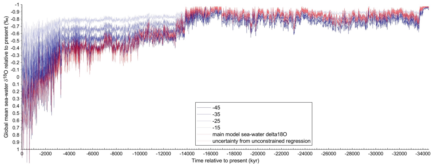
Supplementary Figure S7. Sea-level related change in sea-water \delta^{18}\text{O} (i.e., \Delta\delta_w ). Blue lines reflect reconstructions from \Delta\delta_w:\Delta_{SL} relationships based on different mass-weighted mean global \delta_{ice} values ( \delta_{ice}^* ), as specified in the legend (‰). Red lines with shading in between indicate results from the model presented here (regression range as specified in the legend). For ice-volume growth indicated by our regression-based \Delta_{SL} record (Suppl. Fig. S3), Rayleigh-distillation based fractionation of \delta_p for AIS at the EOT evolves rapidly to -30 to -35\% . Assuming more negative initial snow \delta_p but similar \delta_p development for a large-size AIS (i.e., adjusting the intercept in the relationship for AIS in Suppl. Fig. 1) only negligibly shifts the red curve because the ice sheet grows rapidly to mid-size dimensions. Hence, such an assumption yields no feasible solution to the limited \delta_w impact of AIS growth at the EOT.
