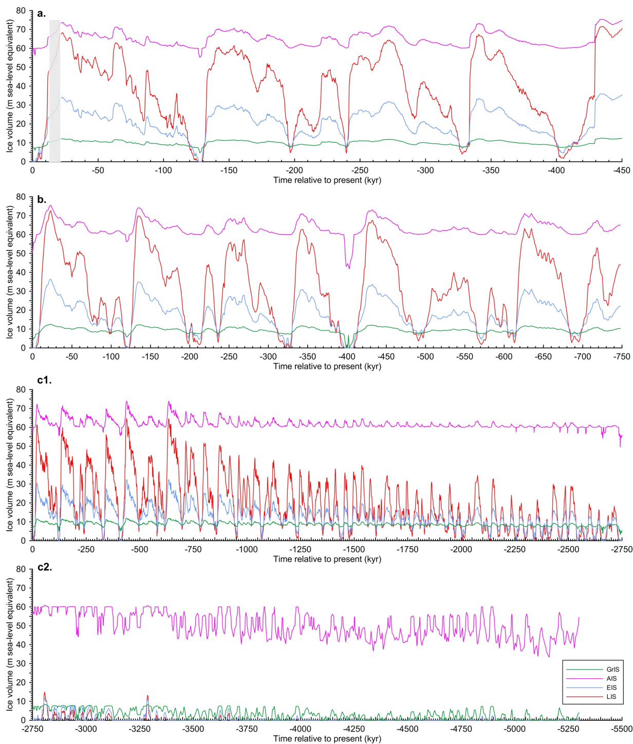
Supplementary Figure S4. Volumes of the various ice sheets. For sea level based on: a. the Red Sea record (8,9,10,11); b. sea-level stack (12); c1 and c2. the benthic \delta_c stack (13) (main case regression, Suppl. Fig. S3). Panel c is divided into younger ( c1 ) and older ( c2 ) halves, for clarity.
