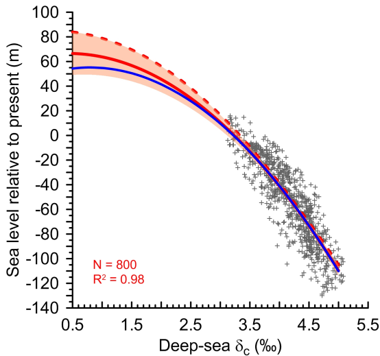
Supplementary Figure S3. Lag-optimized (12) regressions between the benthic foraminiferal carbonate \delta^{18}\text{O} stack (13) and sea-level (12). Second order polynomials are used (12). The solid red line is our main-case conversion regression, which is constrained to peak at 65.1 m. The shaded band indicates its 95% confidence interval, which includes both uncertainty in the regression through the dataset, and normally distributed uncertainties in both X and Y directions for all data points, with 1\sigma = 0.1 ‰ for \delta_c and 1\sigma = 2 m for \Delta_{SL} . For an upper extreme, we use the upper 95% line (dashed red). For a lower extreme, we use the unconstrained second-order polynomial (solid blue). This line peaks at about 55 m and, thus, always “leaves” about 10 m of ice, which is unrealistic. Thus, we ignored the lower 95% bound of the main regression because that remains even lower. Main line equation (solid red): \Delta_{SL} = -8.4 \delta_c^2 + 6.8 \delta_c + 65.1 . Upper 95% bound equation (dashed red): \Delta_{SL} = -7.8 \delta_c^2 + 0.1 \delta_c + 86.2 . Unconstrained polynomial equation (solid blue): \Delta_{SL} = -9.3 \delta_c^2 + 14.3 \delta_c + 50.4 . Statistics given in the figure refer to the main polynomial.
