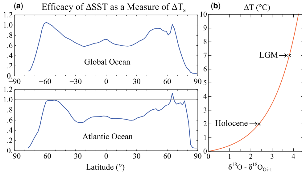
Figure 7. (a) Ratio of \Delta S_{ST} (latitude) to global T_S change for all ocean and the Atlantic Ocean, based on equilibrium response (years 4001–4500) in 2 \times CO_2 simulations of GISS (2020) model. (b) \Delta T , the amount by which T_S change exceeds T_{do} change, based on an exponential fit to the two data points provided by the Holocene and LGM (see text).
