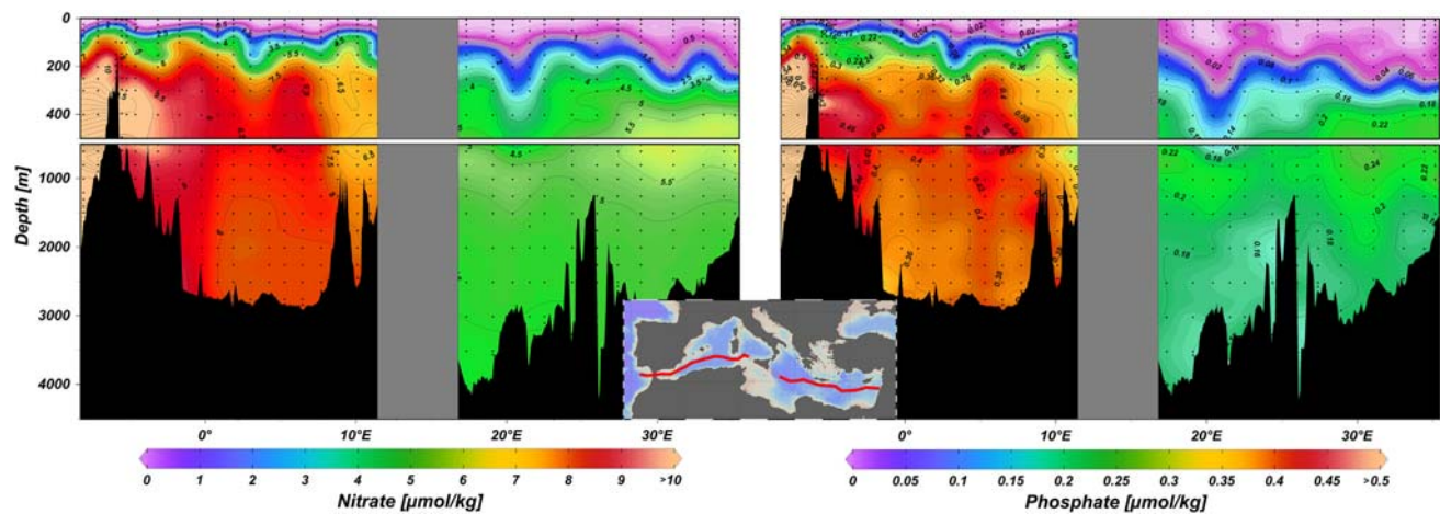
FIGURE 11.5 Vertical distribution of nitrate (left) and phosphate (right), in \mu\text{mol kg}^{-1} , along a trans-Mediterranean Sea section (RV METEOR cruise M84/3 in April 2011, see also Tanhua et al., 2013b ).
